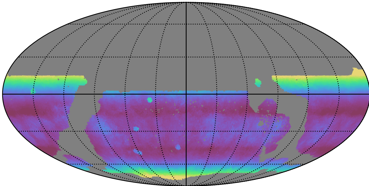
ddf_loaded_half_fl2_v3.4_10yrs WFD r band: Median airmass
