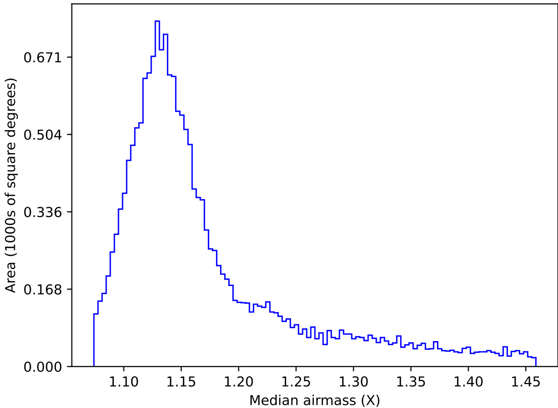
ddf_loaded_half_fl2_v3.4_10yrs WFD r band: Median airmass
