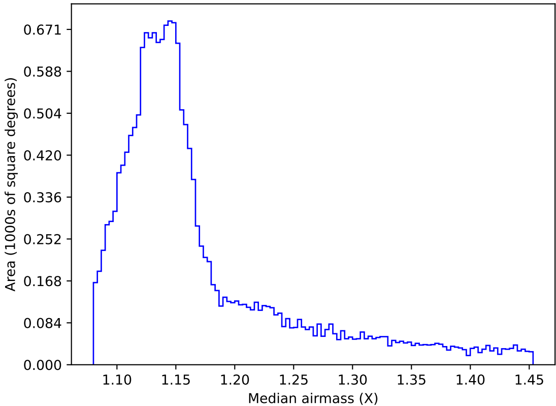
ddf_loaded_half_fl2_v3.4_10yrs WFD i band: Median airmass
