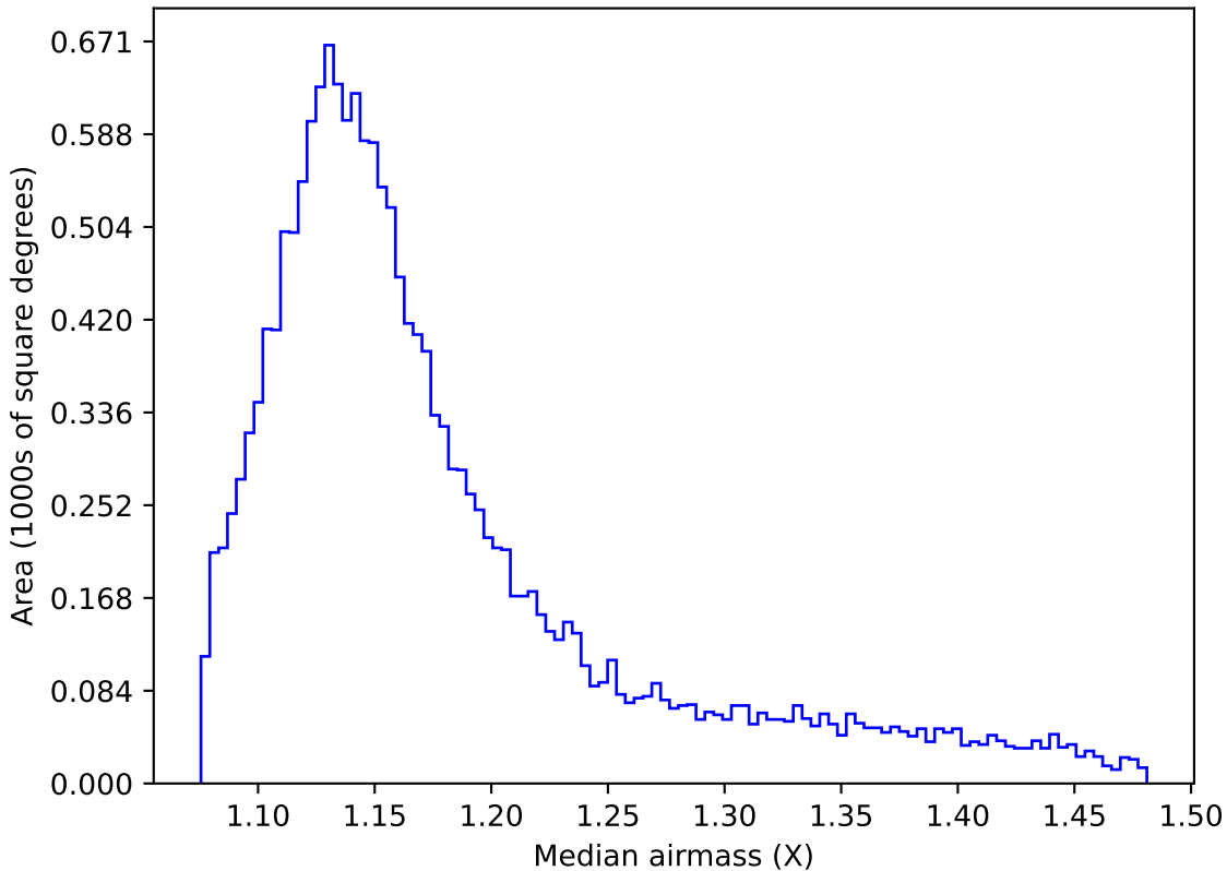
ddf_loaded_half_fl2_v3.4_10yrs WFD g band: Median airmass
