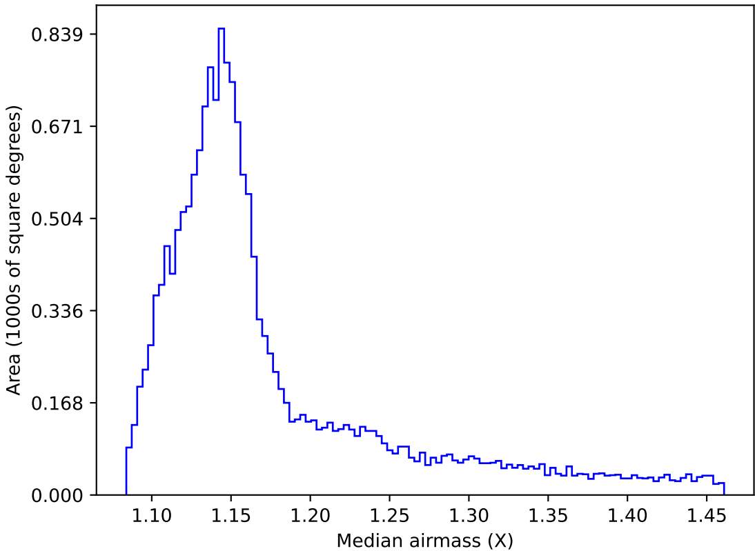
ddf_loaded_half_fl2_v3.4_10yrs WFD all bands: Median airmass
