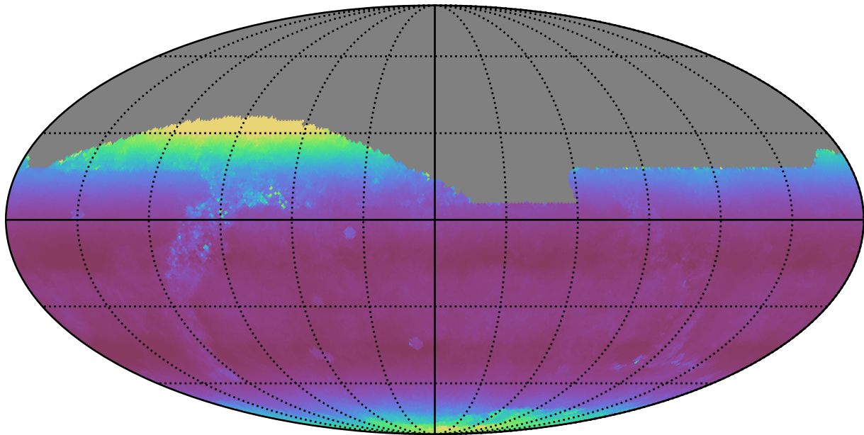
ddf_loaded_half_fl2_v3.4_10yrs All sky z band: Median airmass
