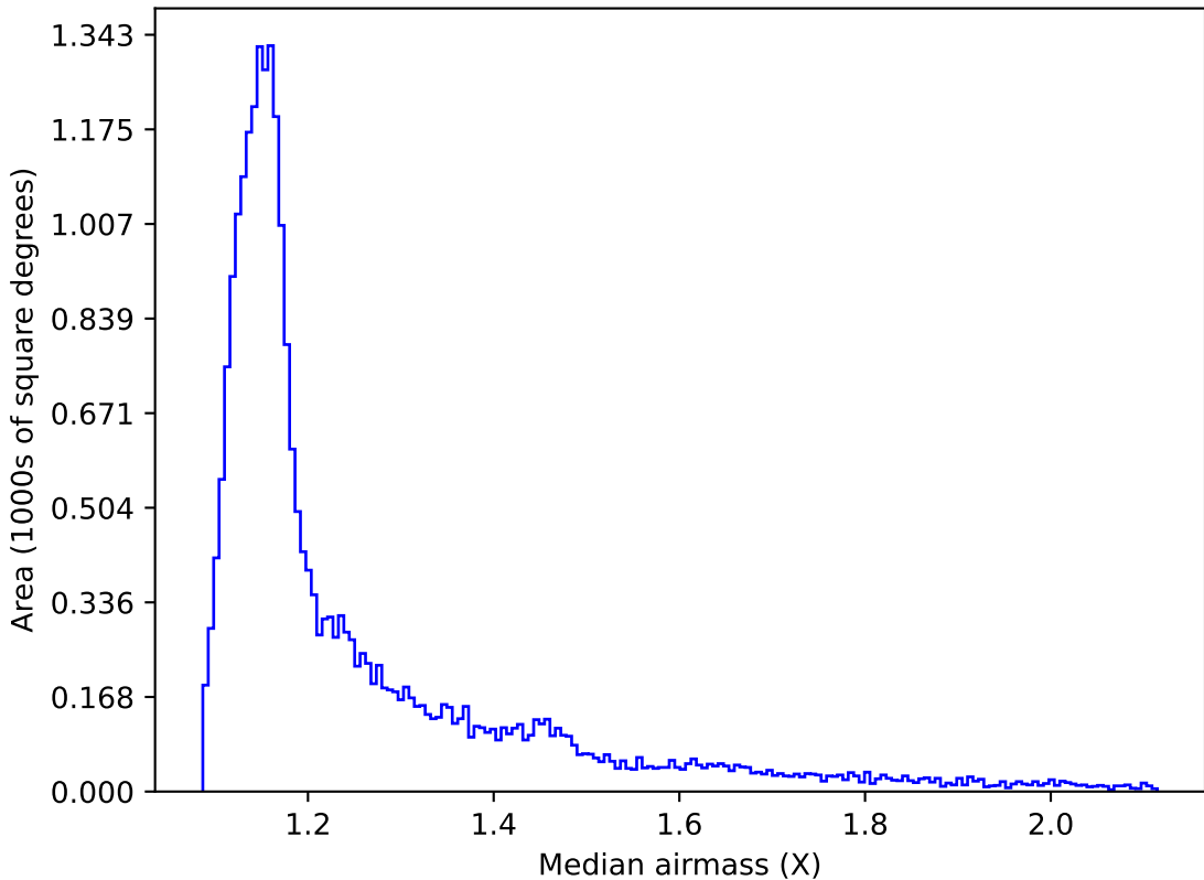
ddf_loaded_half_fl2_v3.4_10yrs All sky z band: Median airmass
