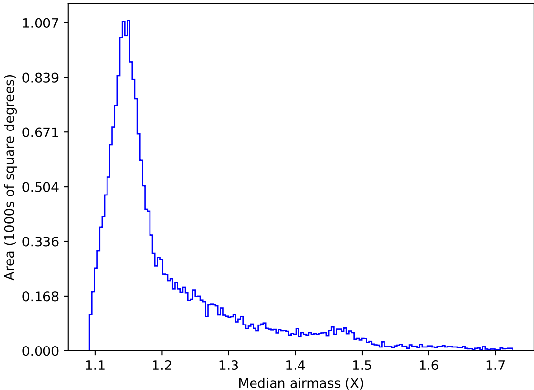
ddf_loaded_half_fl2_v3.4_10yrs All sky y band: Median airmass
