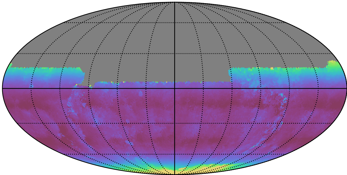
ddf_loaded_half_f12_v3.4_10yrs All sky u band: Median airmass
