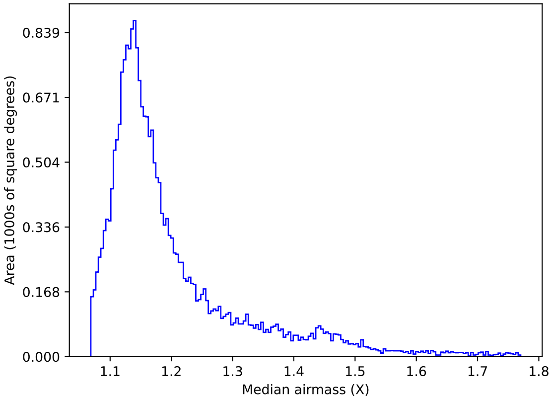
ddf_loaded_half_fl2_v3.4_10yrs All sky u band: Median airmass
