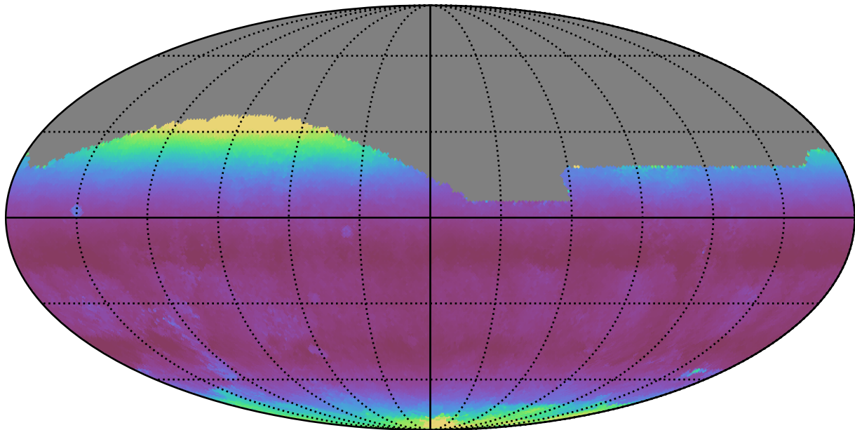
ddf_loaded_half_fl2_v3.4_10yrs All sky g band: Median airmass
