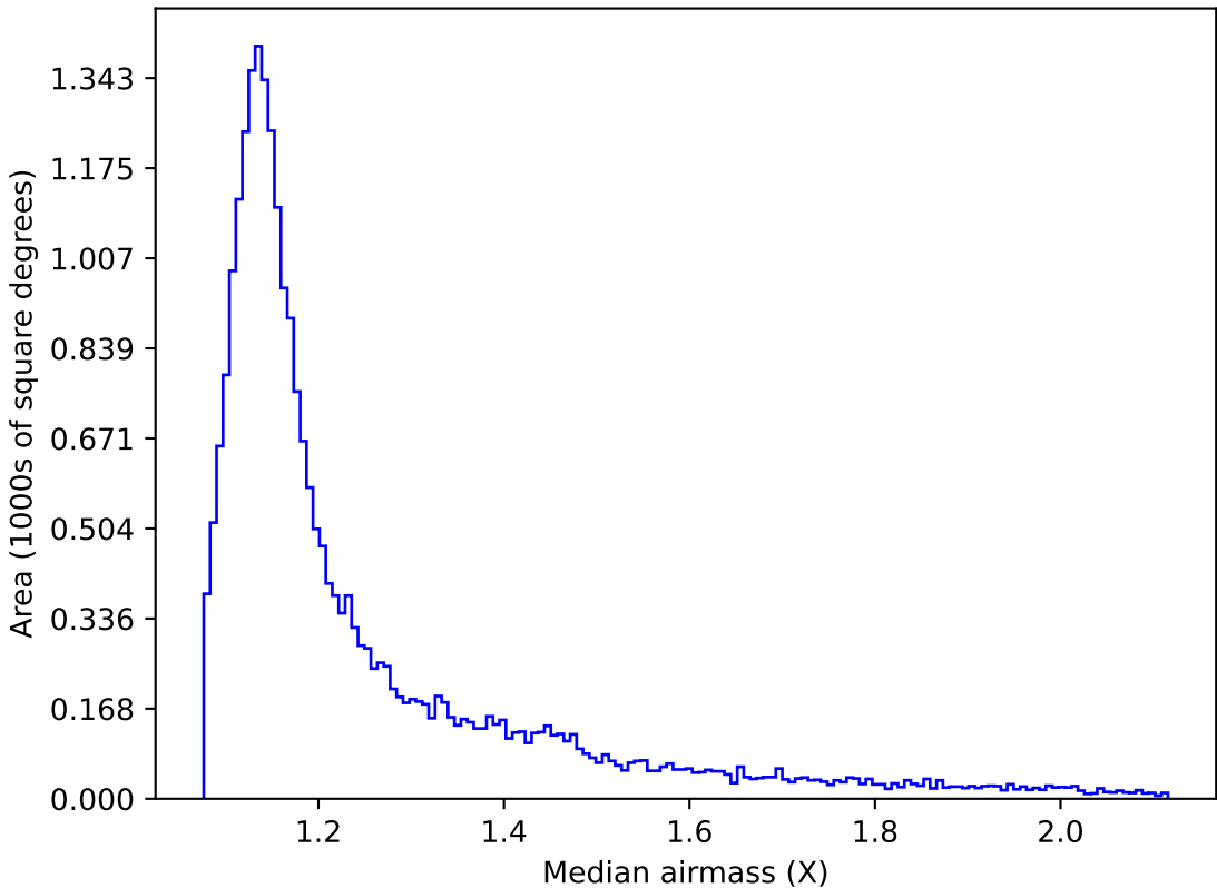
ddf_loaded_half_fl2_v3.4_10yrs All sky g band: Median airmass
