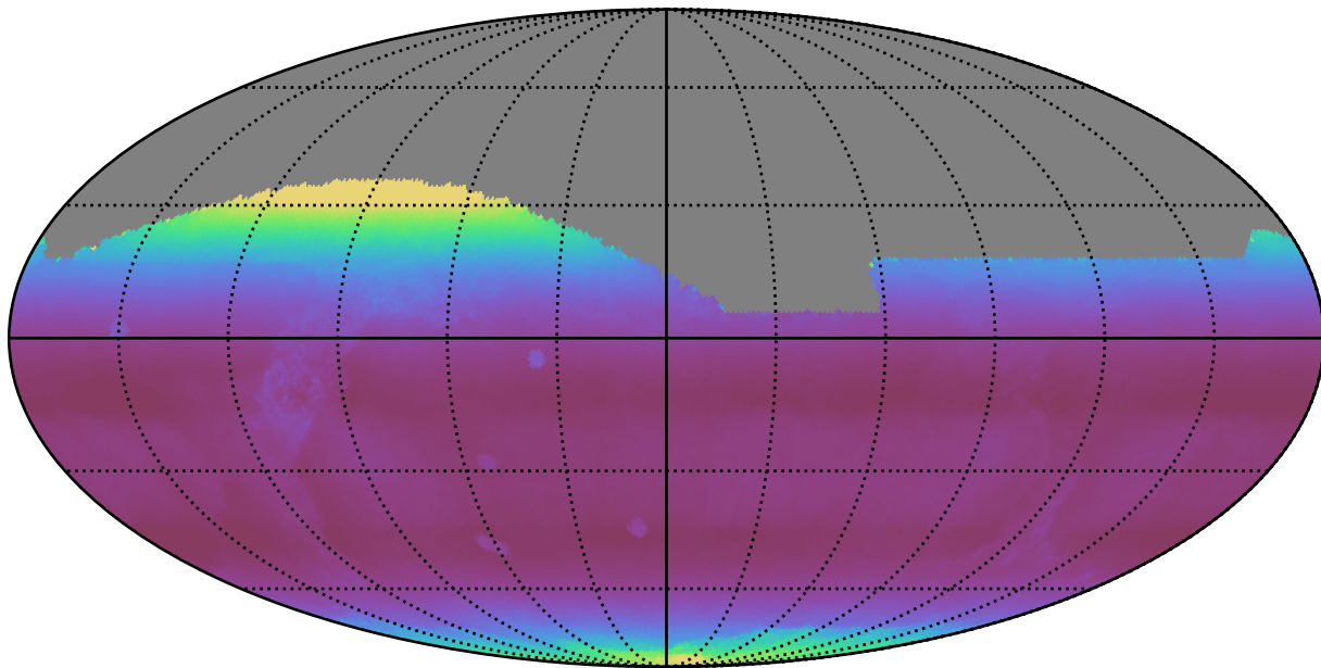
ddf_loaded_half_fl2_v3.4_10yrs All sky all bands: Median airmass
