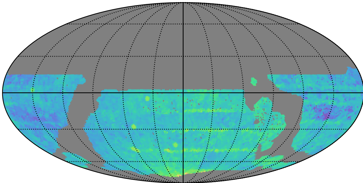
ddf_loaded_half_fl2_v3.4_10yrs WFD z band: Median Season Length
