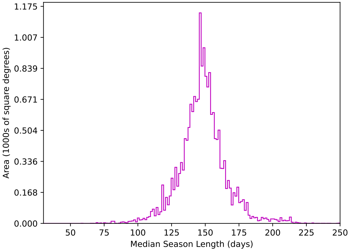
ddf_loaded_half_fl2_v3.4_10yrs WFD z band: Median Season Length
