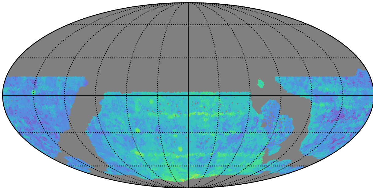
ddf_loaded_half_fl2_v3.4_10yrs WFD y band: Median Season Length
