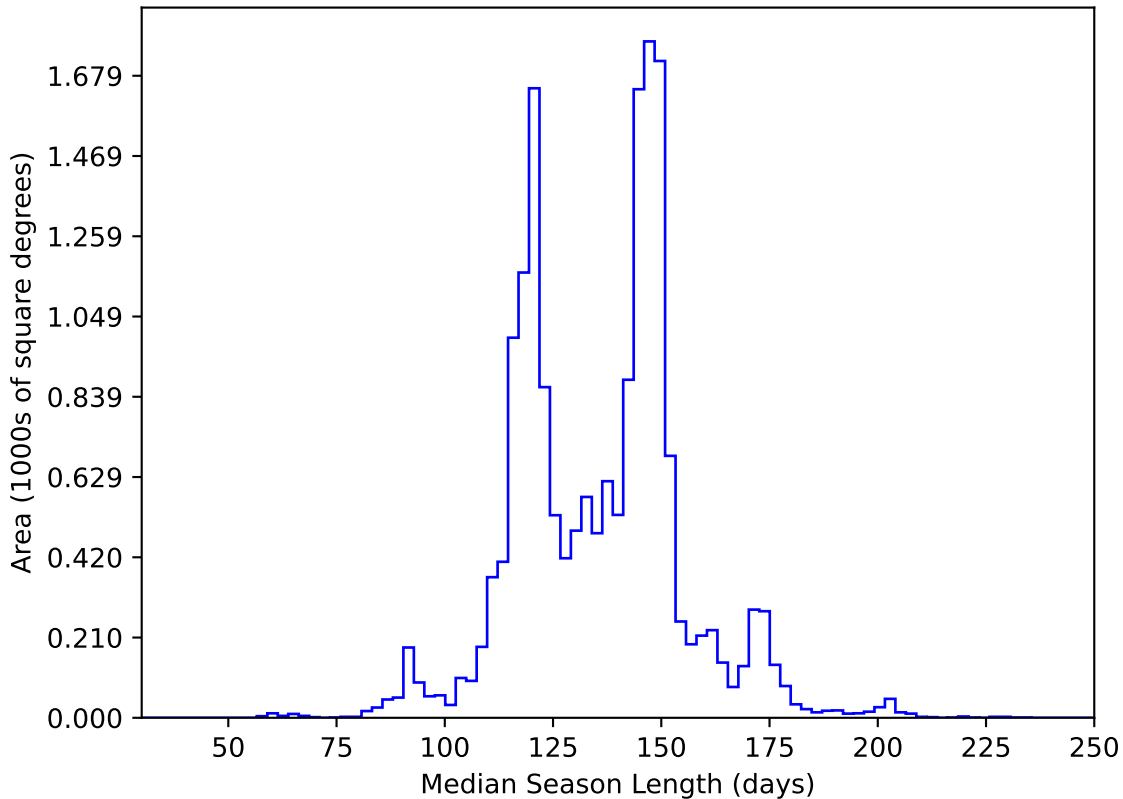
ddf_loaded_half_fl2_v3.4_10yrs WFD y band: Median Season Length
