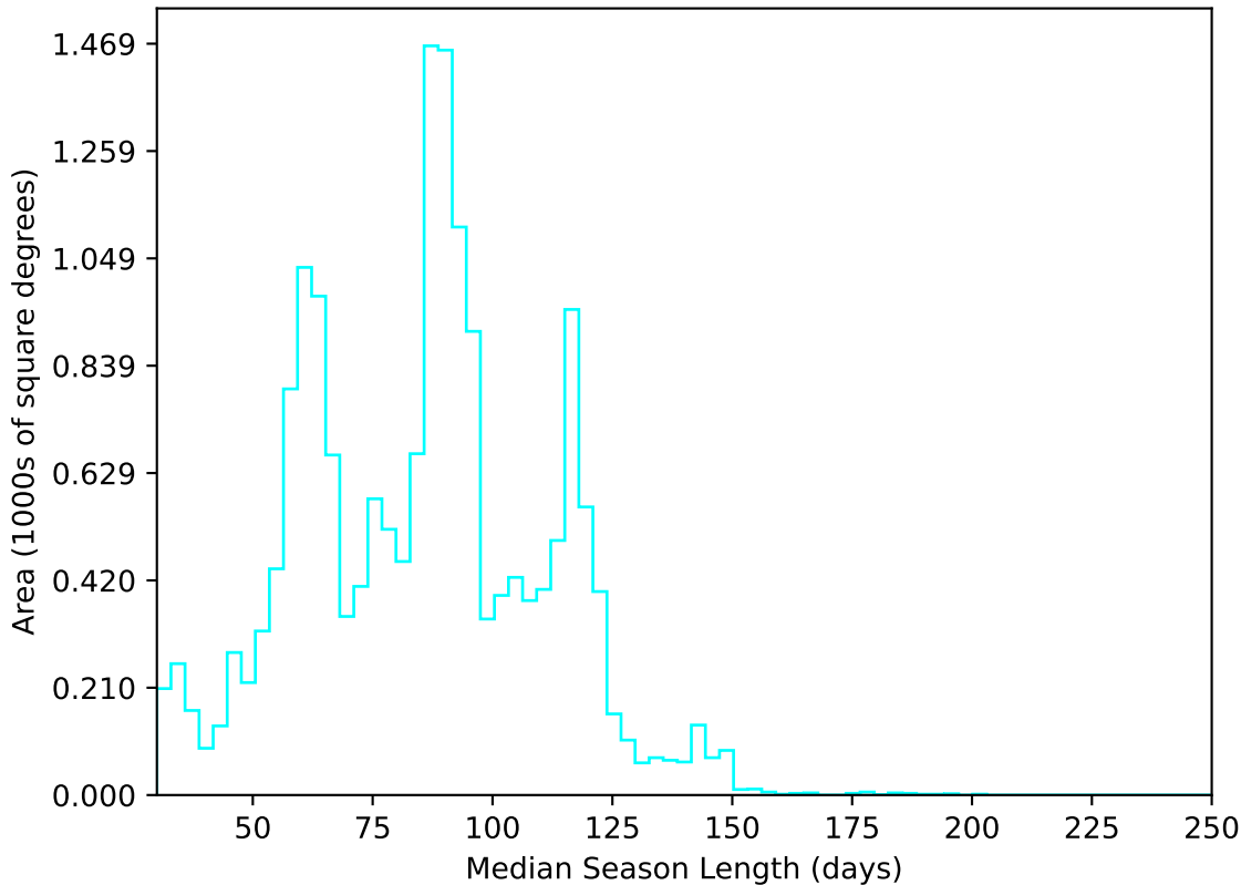
ddf_loaded_half_fl2_v3.4_10yrs WFD u band: Median Season Length
