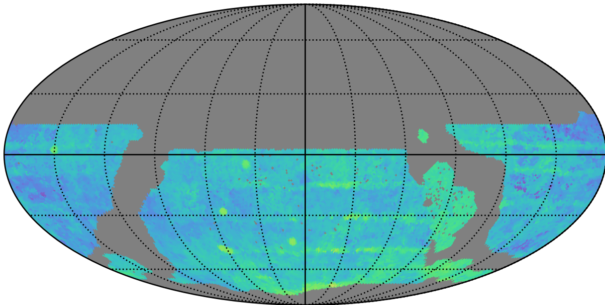
ddf_loaded_half_fl2_v3.4_10yrs WFD r band: Median Season Length
