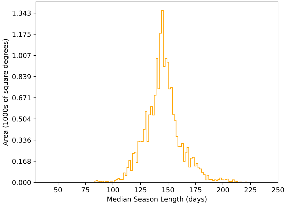
ddf_loaded_half_fl2_v3.4_10yrs WFD r band: Median Season Length
