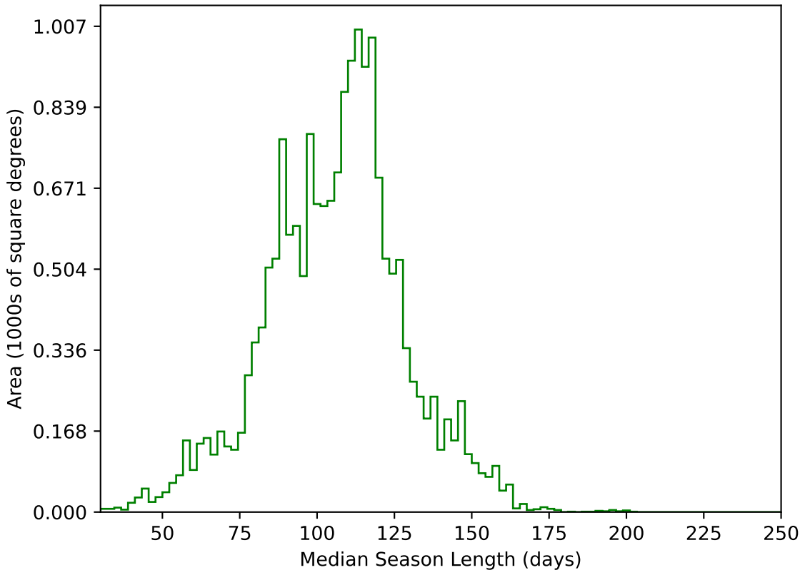
ddf_loaded_half_fl2_v3.4_10yrs WFD g band: Median Season Length
