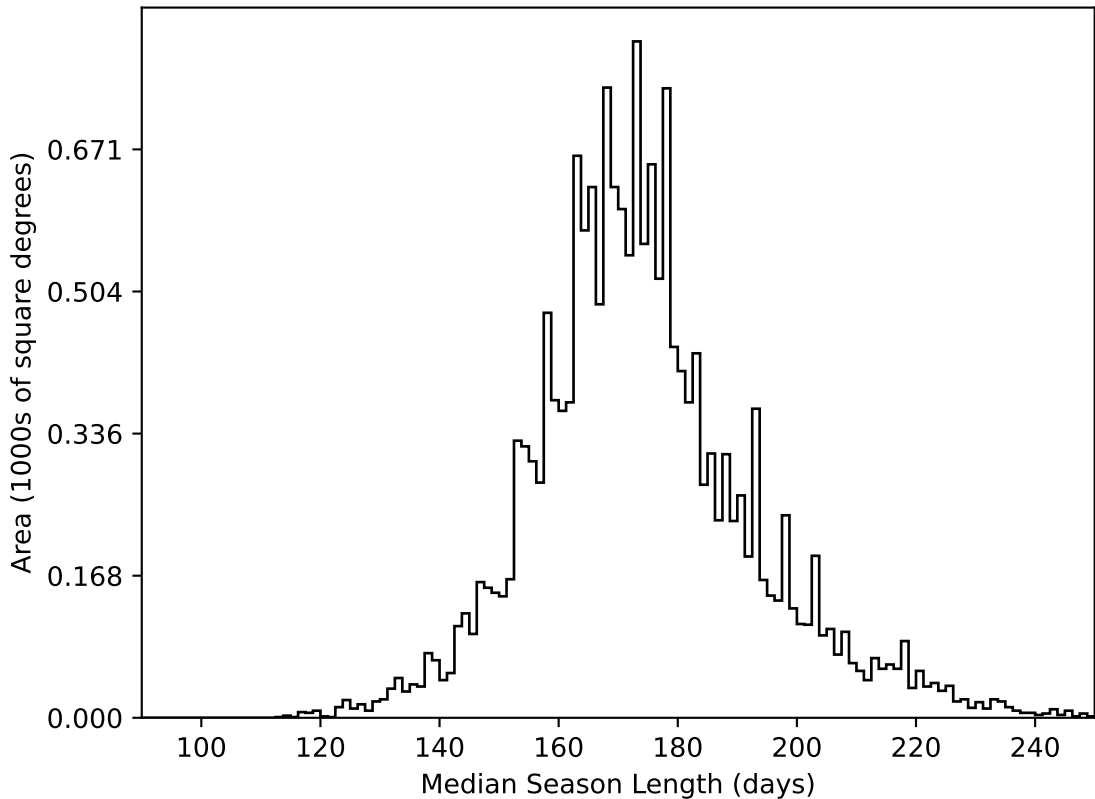
ddf_loaded_half_fl2_v3.4_10yrs WFD all bands: Median Season Length
