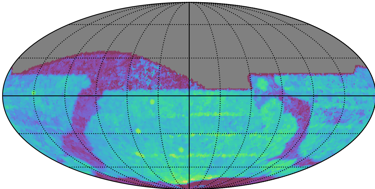
ddf_loaded_half_fl2_v3.4_10yrs All sky z band: Median Season Length
