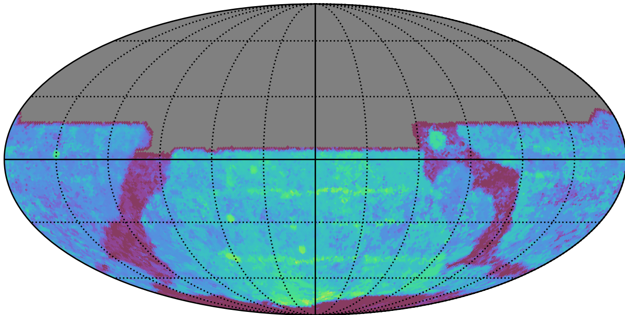
ddf_loaded_half_fl2_v3.4_10yrs All sky y band: Median Season Length
