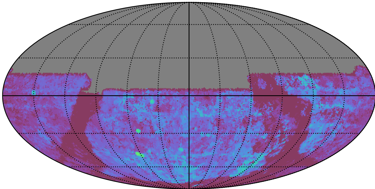
ddf_loaded_half_f12_v3.4_10yrs All sky u band: Median Season Length
