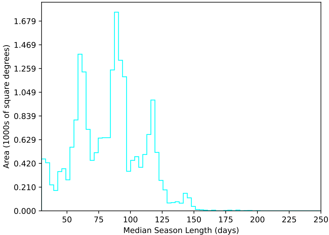
ddf_loaded_half_fl2_v3.4_10yrs All sky u band: Median Season Length
