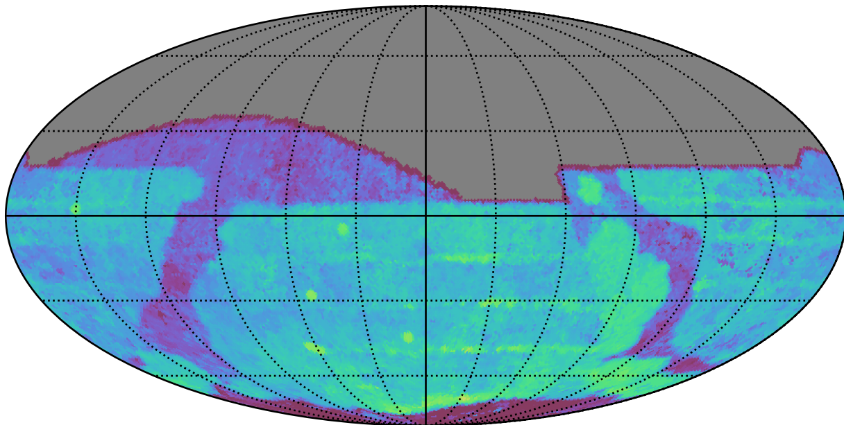
ddf_loaded_half_fl2_v3.4_10yrs All sky r band: Median Season Length
