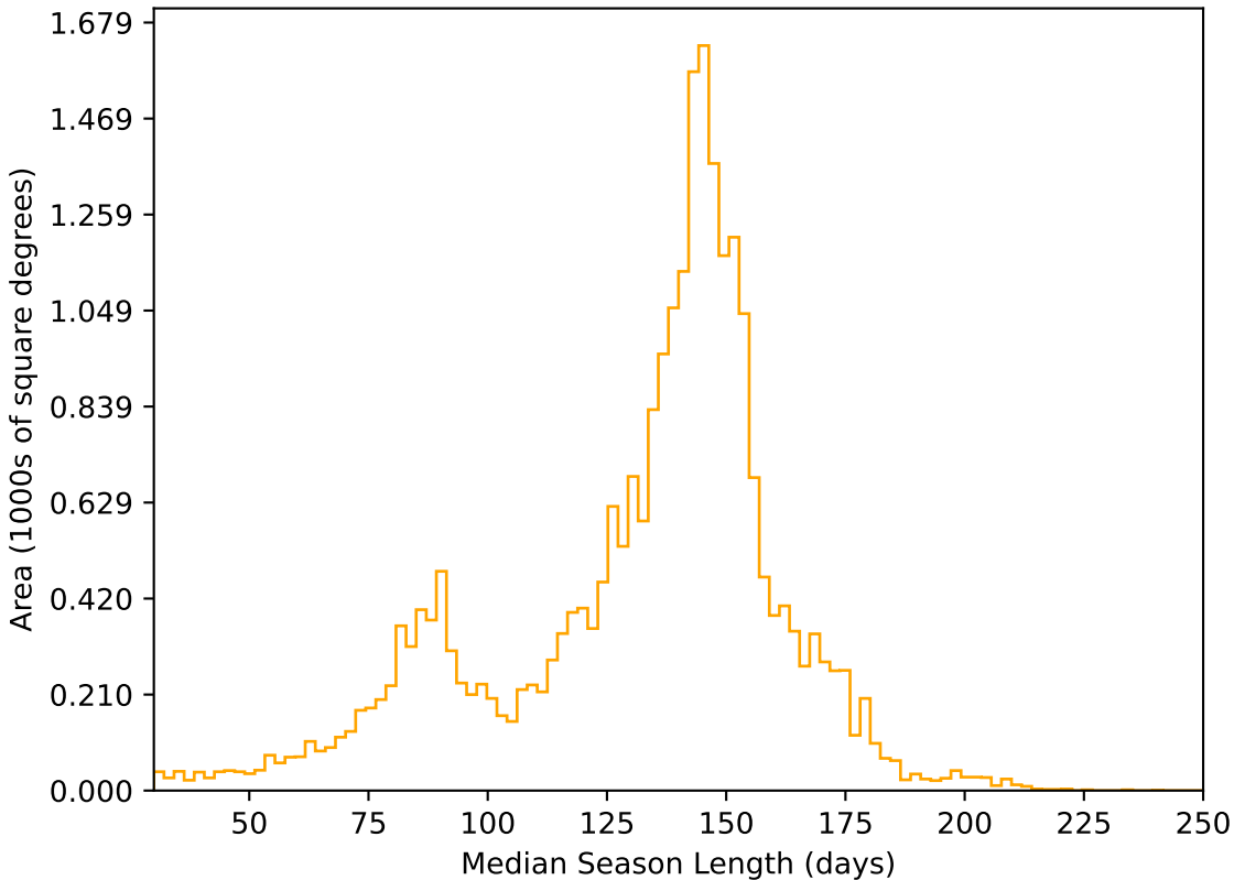
ddf_loaded_half_fl2_v3.4_10yrs All sky r band: Median Season Length
