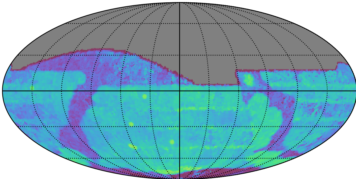
ddf_loaded_half_fl2_v3.4_10yrs All sky i band: Median Season Length
