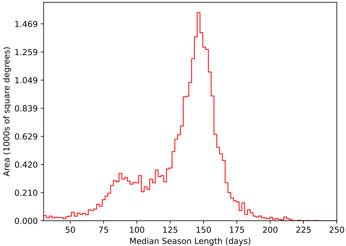
ddf_loaded_half_fl2_v3.4_10yrs All sky i band: Median Season Length
