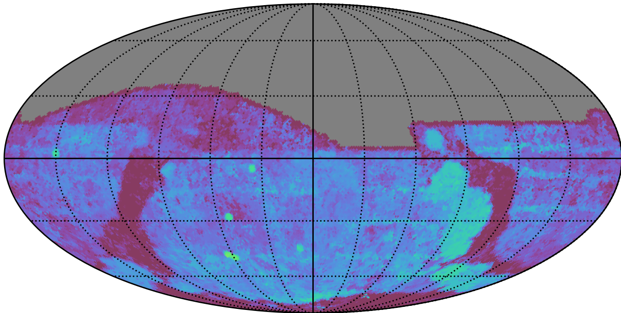
ddf_loaded_half_fl2_v3.4_10yrs All sky g band: Median Season Length
