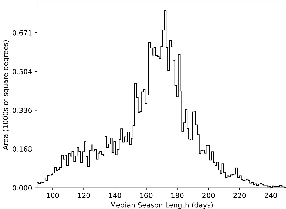
ddf_loaded_half_fl2_v3.4_10yrs All sky all bands: Median Season Length
