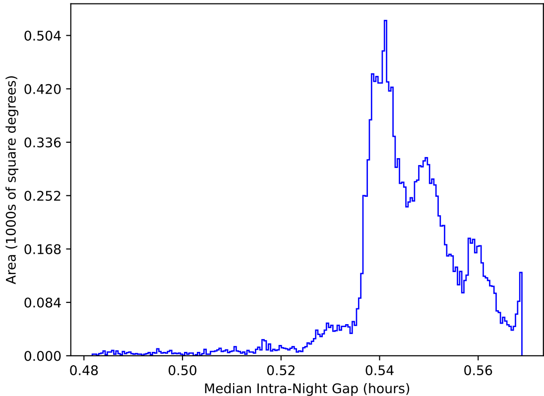
ddf_loaded_half_fl2_v3.4_10yrs WFD: Median Intra-Night Gap
