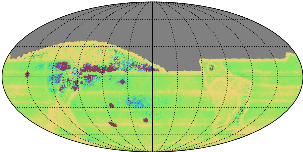
ddf_loaded_half_fl2_v3.4_10yrs All sky: Median Intra-Night Gap
