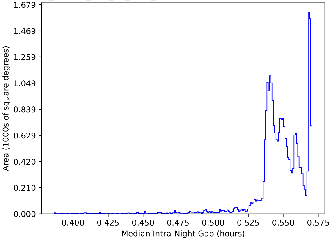
ddf_loaded_half_fl2_v3.4_10yrs All sky: Median Intra-Night Gap
