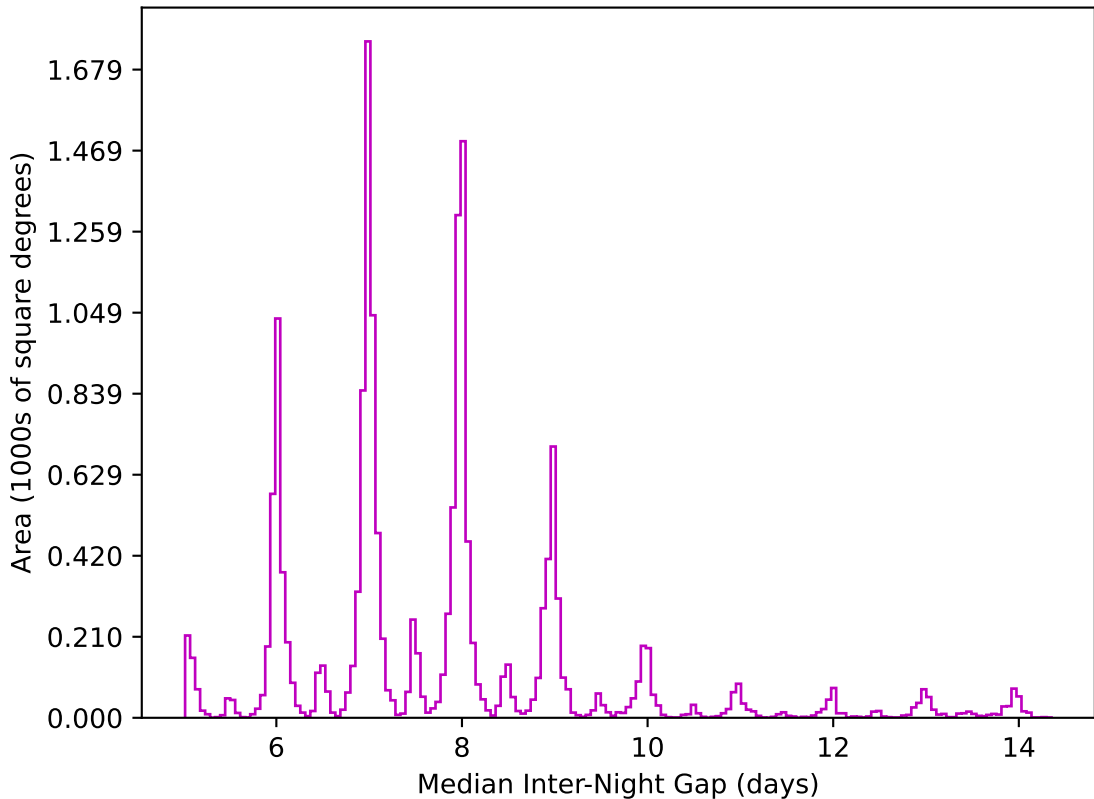
ddf_loaded_half_fl2_v3.4_10yrs WFD z band: Median Inter-Night Gap
