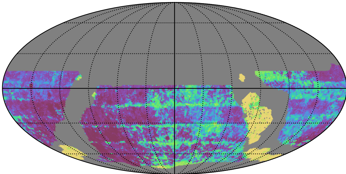
ddf_loaded_half_fl2_v3.4_10yrs WFD y band: Median Inter-Night Gap
