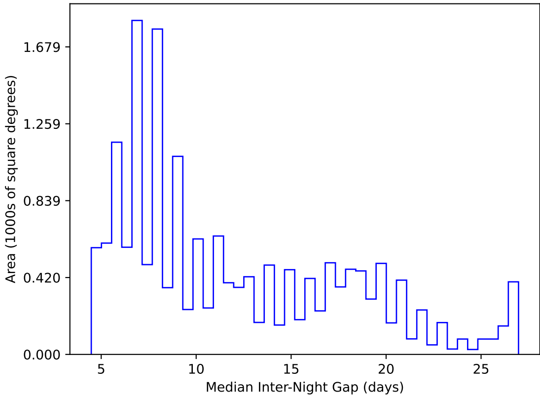
ddf_loaded_half_fl2_v3.4_10yrs WFD y band: Median Inter-Night Gap
