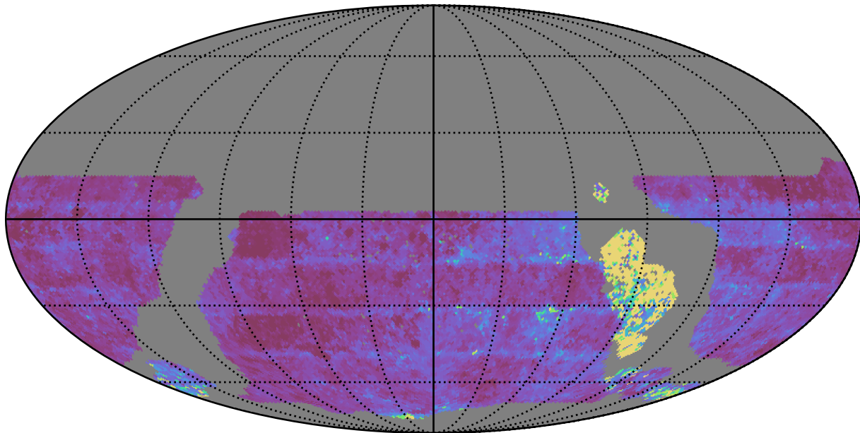
ddf_loaded_half_fl2_v3.4_10yrs WFD u band: Median Inter-Night Gap
