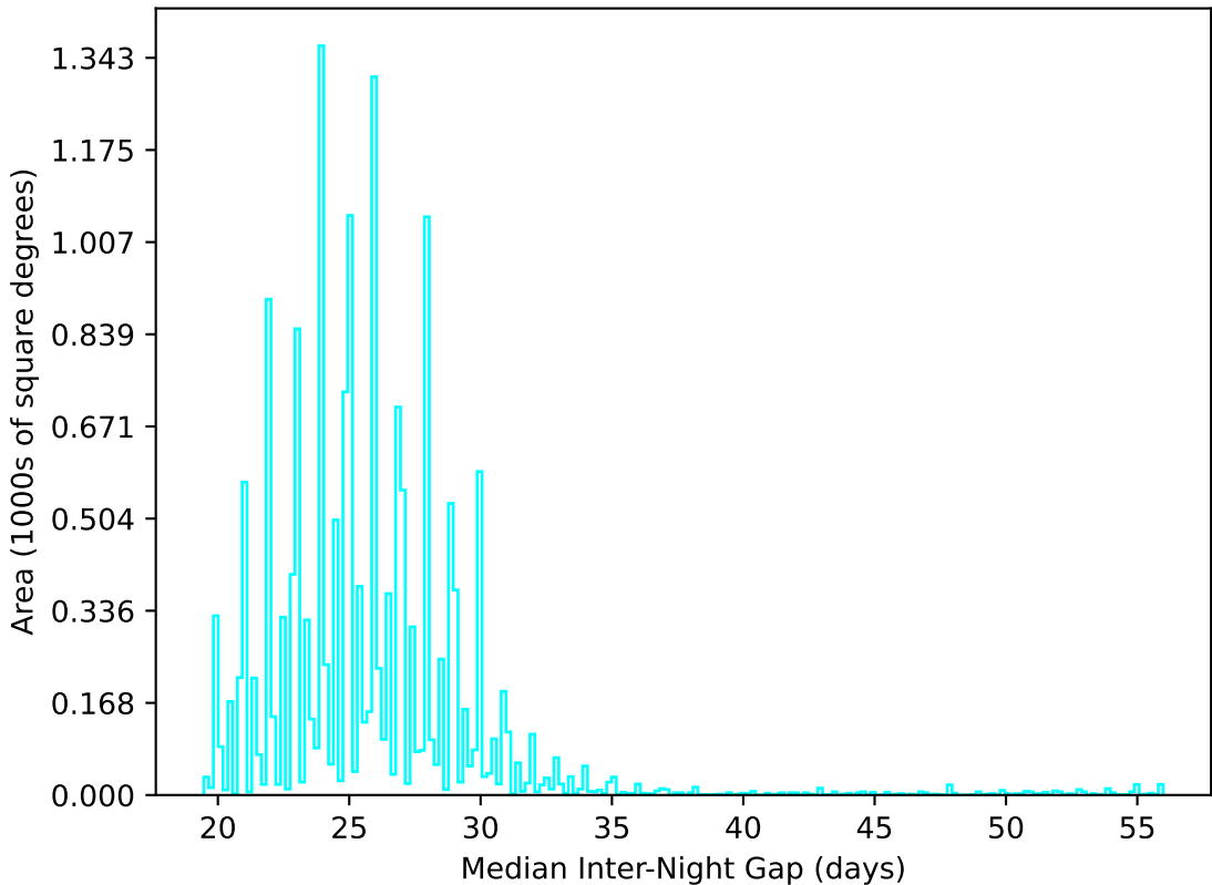
ddf_loaded_half_fl2_v3.4_10yrs WFD u band: Median Inter-Night Gap
