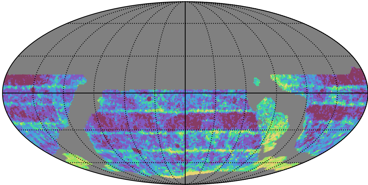
ddf_loaded_half_fl2_v3.4_10yrs WFD r band: Median Inter-Night Gap
