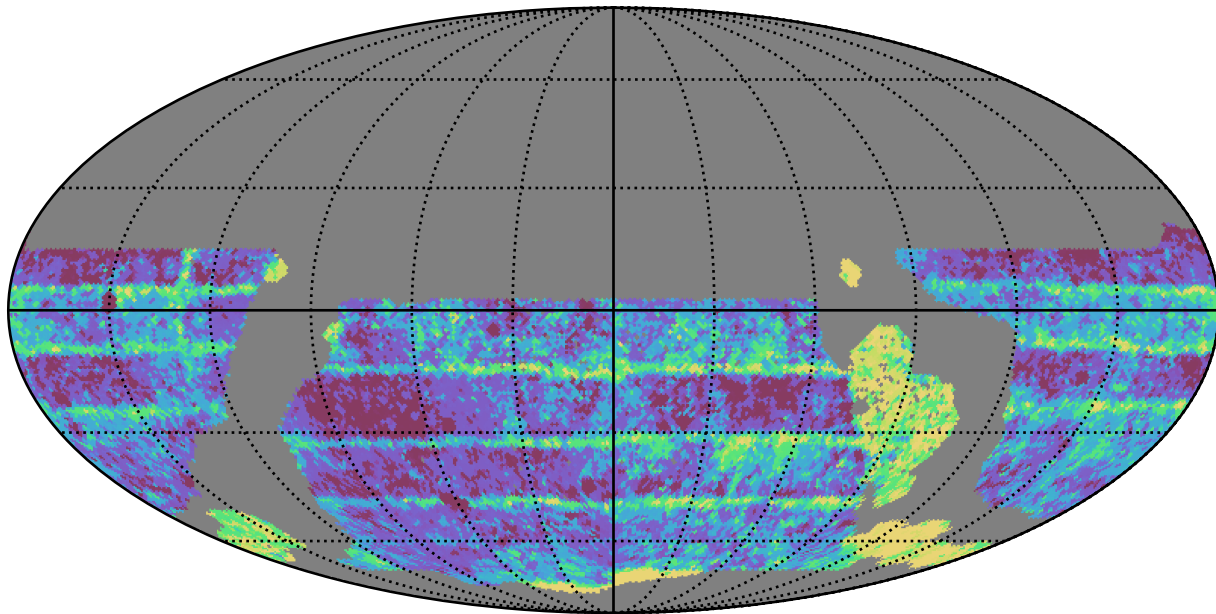
ddf_loaded_half_fl2_v3.4_10yrs WFD i band: Median Inter-Night Gap
