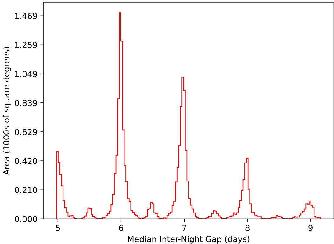
ddf_loaded_half_fl2_v3.4_10yrs WFD i band: Median Inter-Night Gap
