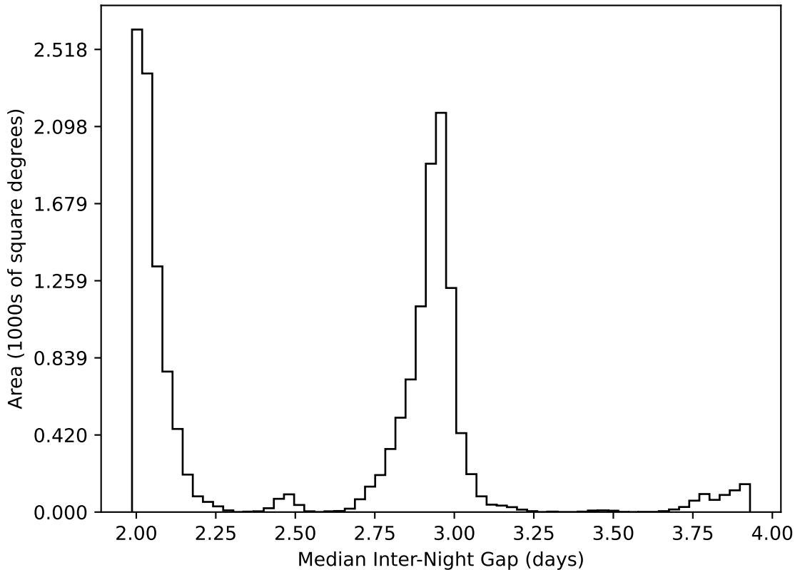
ddf_loaded_half_fl2_v3.4_10yrs WFD all bands: Median Inter-Night Gap
