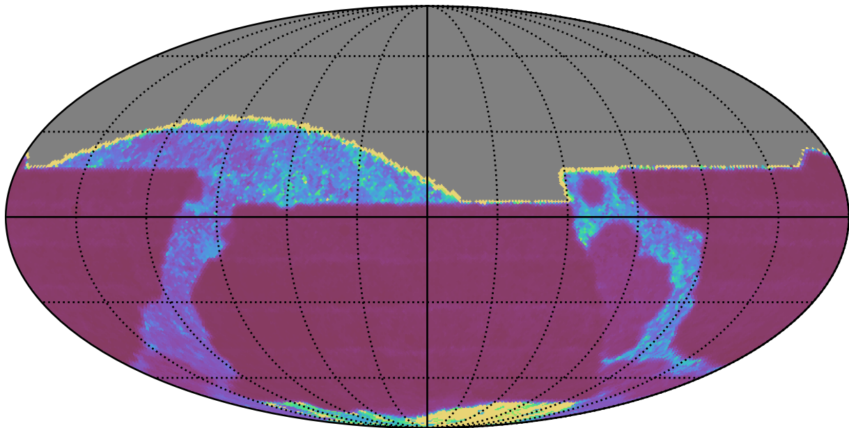
ddf_loaded_half_fl2_v3.4_10yrs All sky z band: Median Inter-Night Gap
