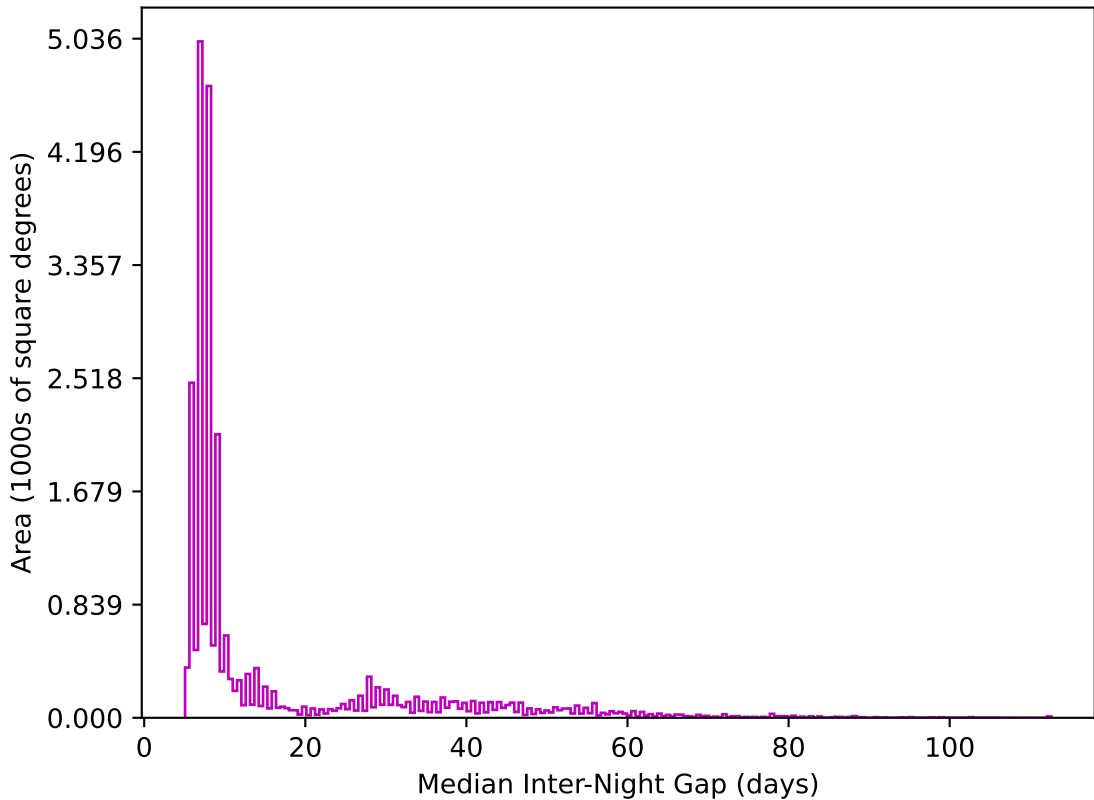
ddf_loaded_half_fl2_v3.4_10yrs All sky z band: Median Inter-Night Gap
