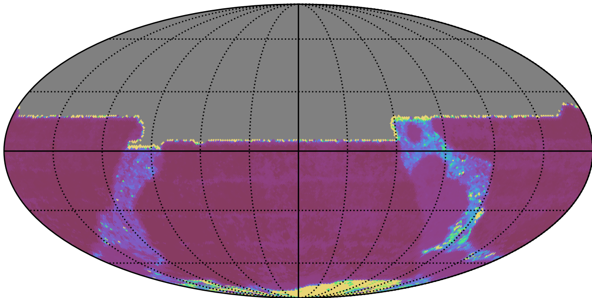
ddf_loaded_half_fl2_v3.4_10yrs All sky y band: Median Inter-Night Gap
