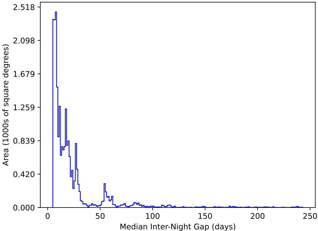
ddf_loaded_half_fl2_v3.4_10yrs All sky y band: Median Inter-Night Gap
