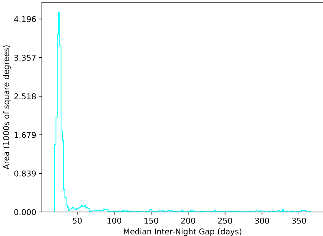
ddf_loaded_half_fl2_v3.4_10yrs All sky u band: Median Inter-Night Gap
