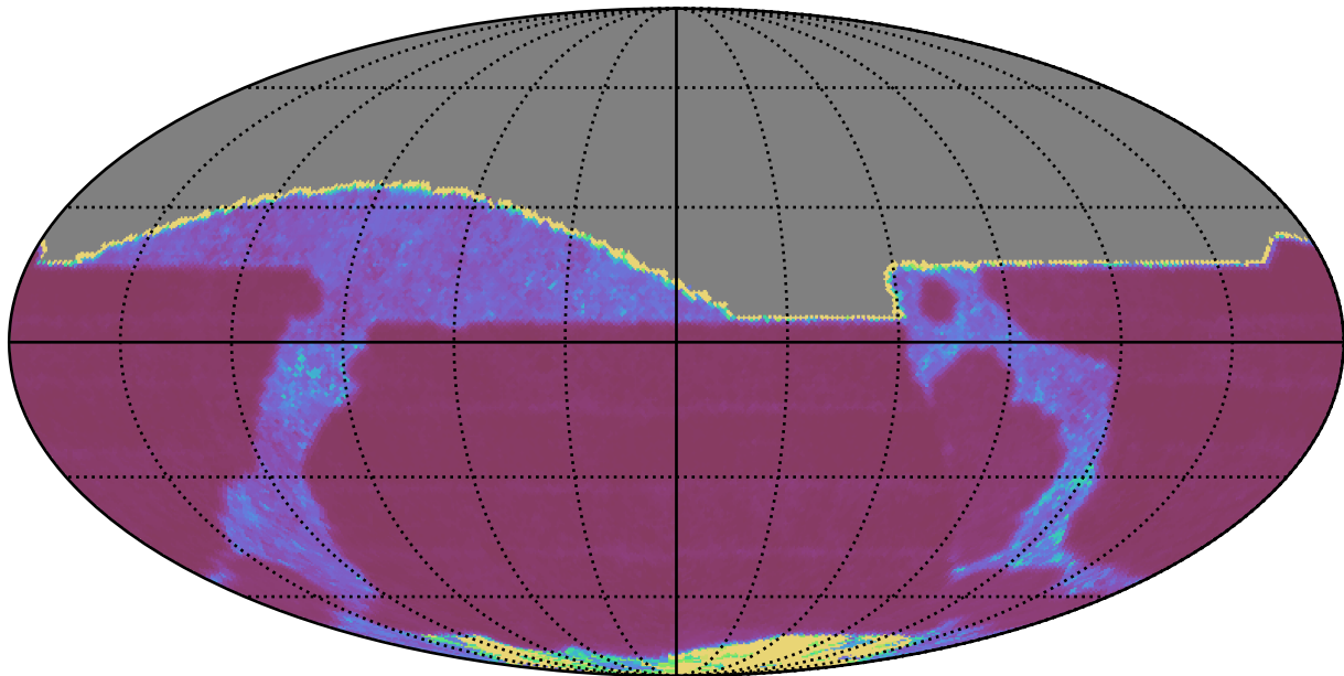
ddf_loaded_half_fl2_v3.4_10yrs All sky r band: Median Inter-Night Gap
